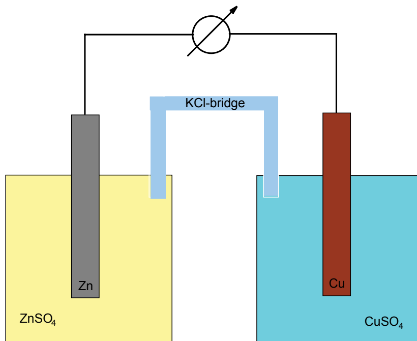
Figure 4.11: Daniell element
