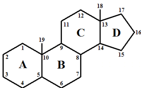
Figure 12.5.1 Steroid Backbone
